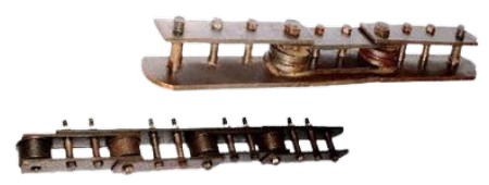
Extractor Chain
